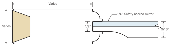
Sample cross section (one-sided mirror door)
